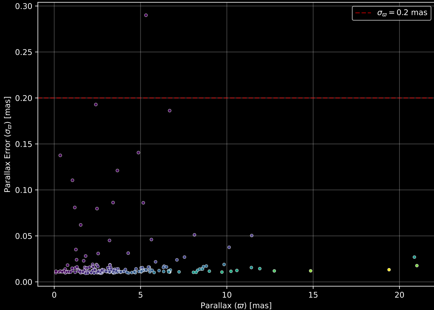
APOGEE DR17 Field: [094+58_MGA] Parallax Quality (n= 220)
