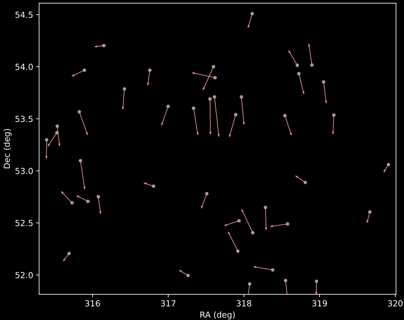
APOGEE DR17 Cluster 7 Proper Motion Vectors (n=43)
