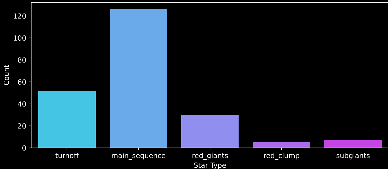
APOGEE DR17 Field: [094+58_MGA] Count plot of Star Type
