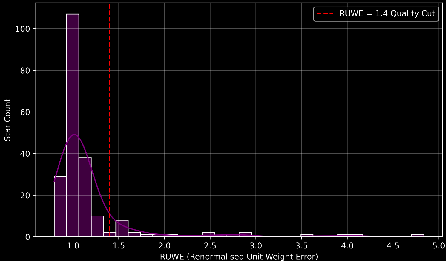
GAPOGEE DR17 Field [094+58_MGA] RUWE Distribution (n= 208)
