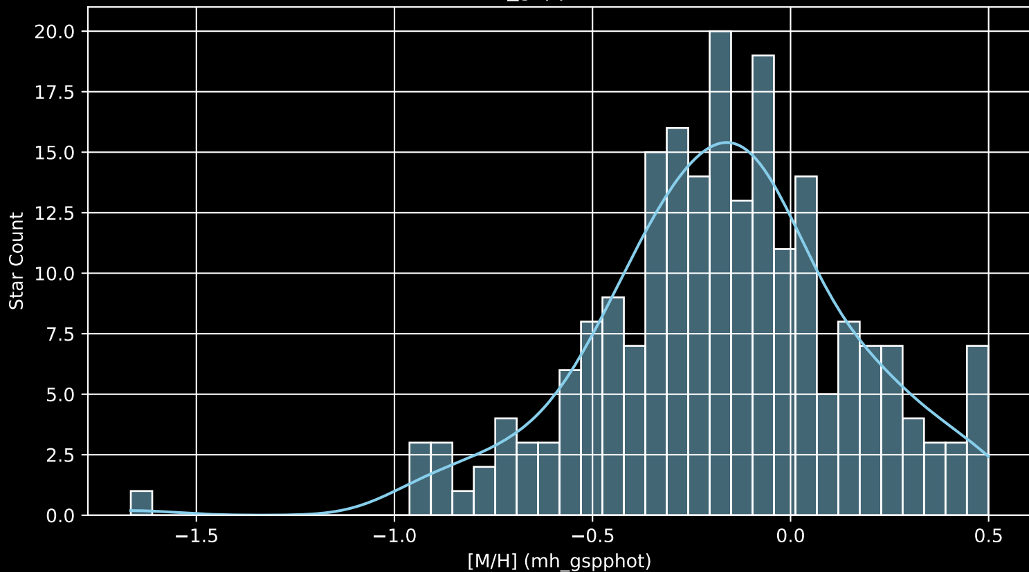
APOGEE DR17 Field: [094+58_MGA [M/H] (mh_gspphot) (n= 216)
