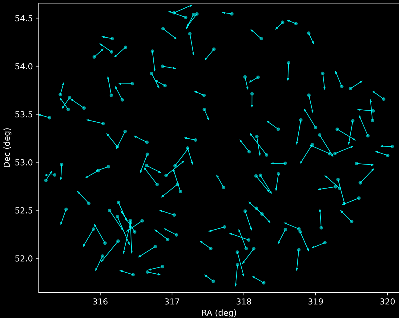
APOGEE DR17 Noise Stream Proper Motion Vectors (n=124)
