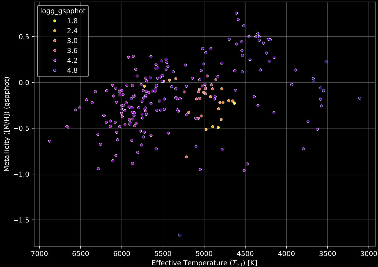
APOGEE DR17 Field: [094+58_MGA] Stellar Population Parameters (n= 220)
