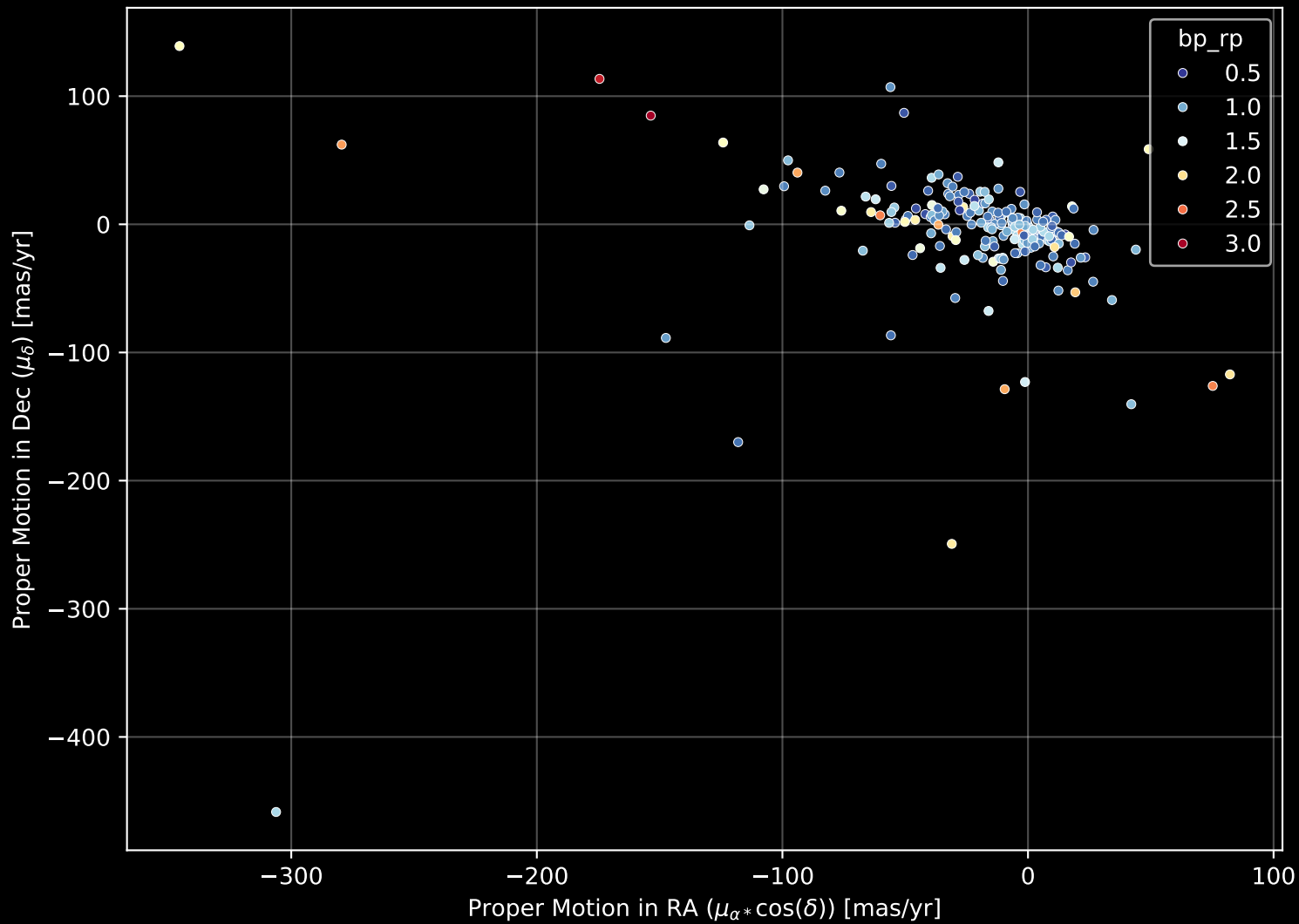
APOGEE DR17 Field: [094+58_MGA] Proper Motion Diagram (n= 220)
